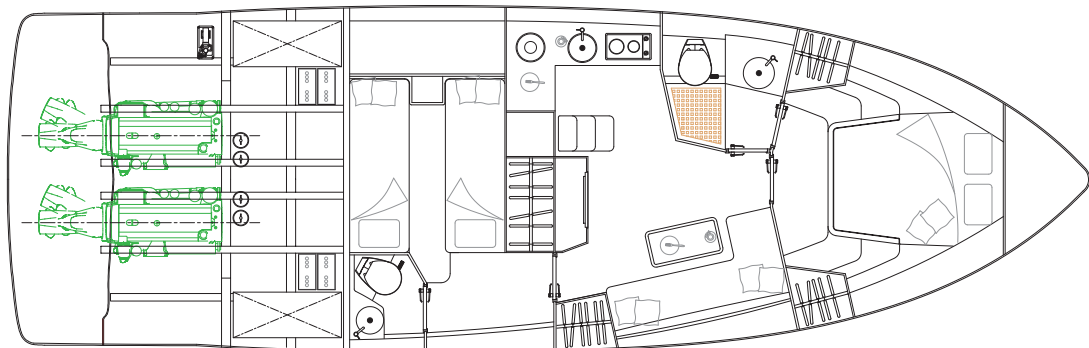
LOWER DECK
