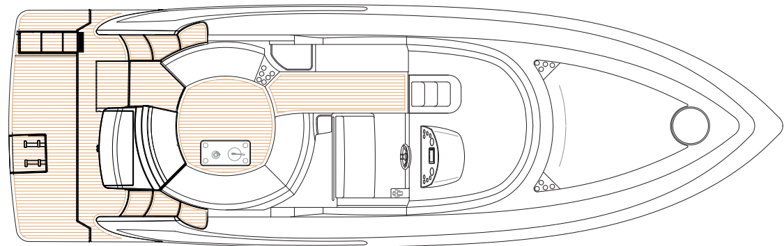
MAIN DECK
