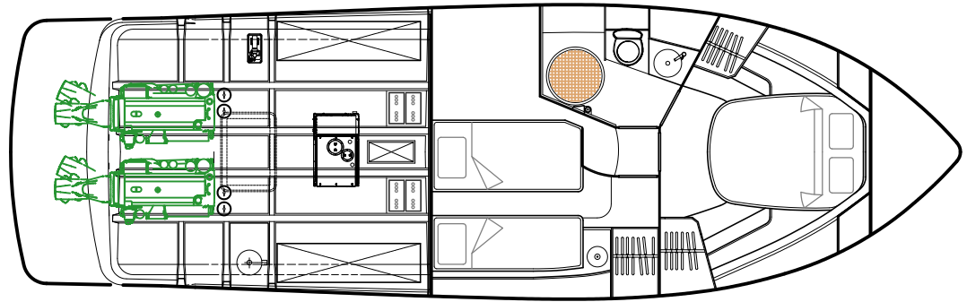
CABINS - OPTION 1
