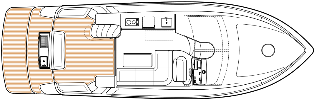
MAIN DECK
