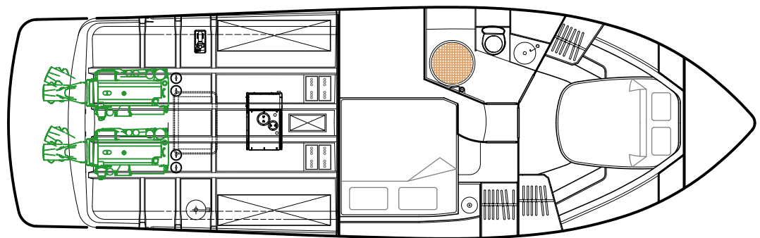
CABINS - OPTION 2
